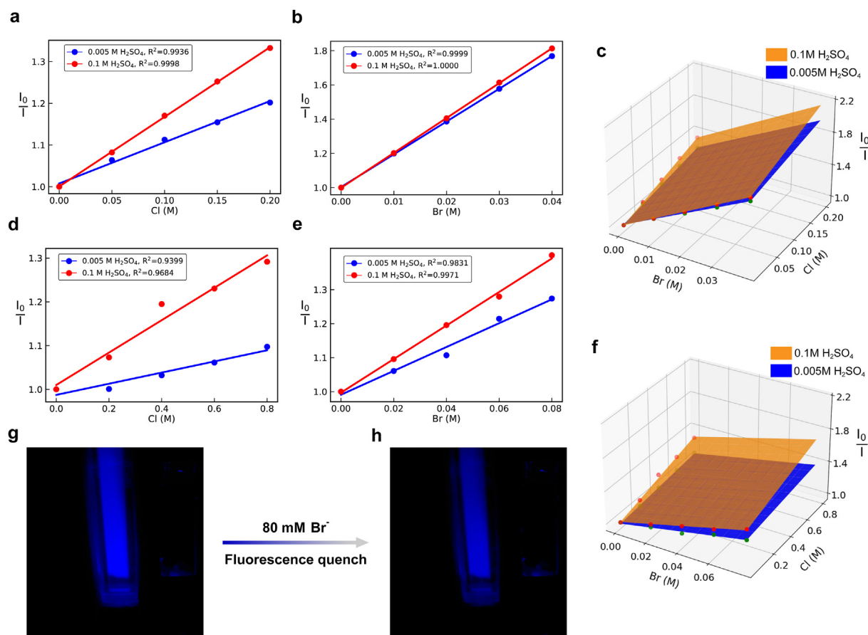
Fig. 4. Standard curves and surfaces of halide(s). (a) Standard curves of \text{Cl}^- at 0.005 M \text{H}_2\text{SO}_4 and 0.1 M \text{H}_2\text{SO}_4 ( R^2 = 0.9936, 0.9998 , respectively) measured using a fluorometer. (b) Standard curves of \text{Br}^- at 0.005 M \text{H}_2\text{SO}_4 and 0.1 M \text{H}_2\text{SO}_4 ( R^2 = 0.9999, 1.0000 , respectively) measured using a fluorometer. (c) Standard surfaces of \text{Cl}^- and \text{Br}^- measured using a fluorometer. (d) Standard curves of \text{Cl}^- at 0.005 M \text{H}_2\text{SO}_4 and 0.1 M \text{H}_2\text{SO}_4 ( R^2 = 0.9399, 0.9684 , respectively) from portable device. (e) Standard curves of \text{Br}^- at 0.005 M \text{H}_2\text{SO}_4 and 0.1 M \text{H}_2\text{SO}_4 ( R^2 = 0.9831, 0.9971 , respectively) from portable device. (f) Standard surfaces of \text{Cl}^- and \text{Br}^- from portable device. (g) Image from portable device with 0 \text{Cl}^- and 0 \text{Br}^- . (h) Image from portable device with 0 \text{Cl}^- and 80 mM \text{Br}^- .
