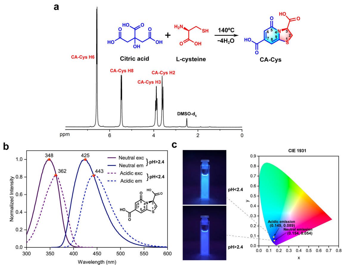
Fig. 2. The synthesis and optical properties of CA-Cys. (a) The one-pot synthesis of CA-Cys from citric acid and L-cysteine; and ^1H NMR spectrum of CA-Cys. (b) The fluorescence spectra of CA-Cys in its neutral ( pH > 2.4 ) and acidic states ( pH < 2.4 ). The pH conditions below 2.4 open the accessibility of CA-Cys to dynamic quenching due to the excited state protonation of 5-carbonyl group. (c) The fluorescence images of CA-Cys in cuvettes and their CIE 1931 chromaticity coordinates at neutral ( pH > 2.4 ) and acidic states ( pH < 2.4 ).
